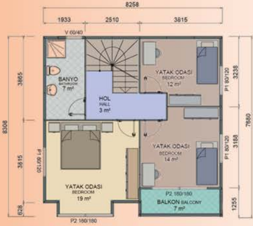
67 m 2 (60 m 2 + 7 m 2 ) 1. KAT PLANI FIRST FLOOR PLAN
